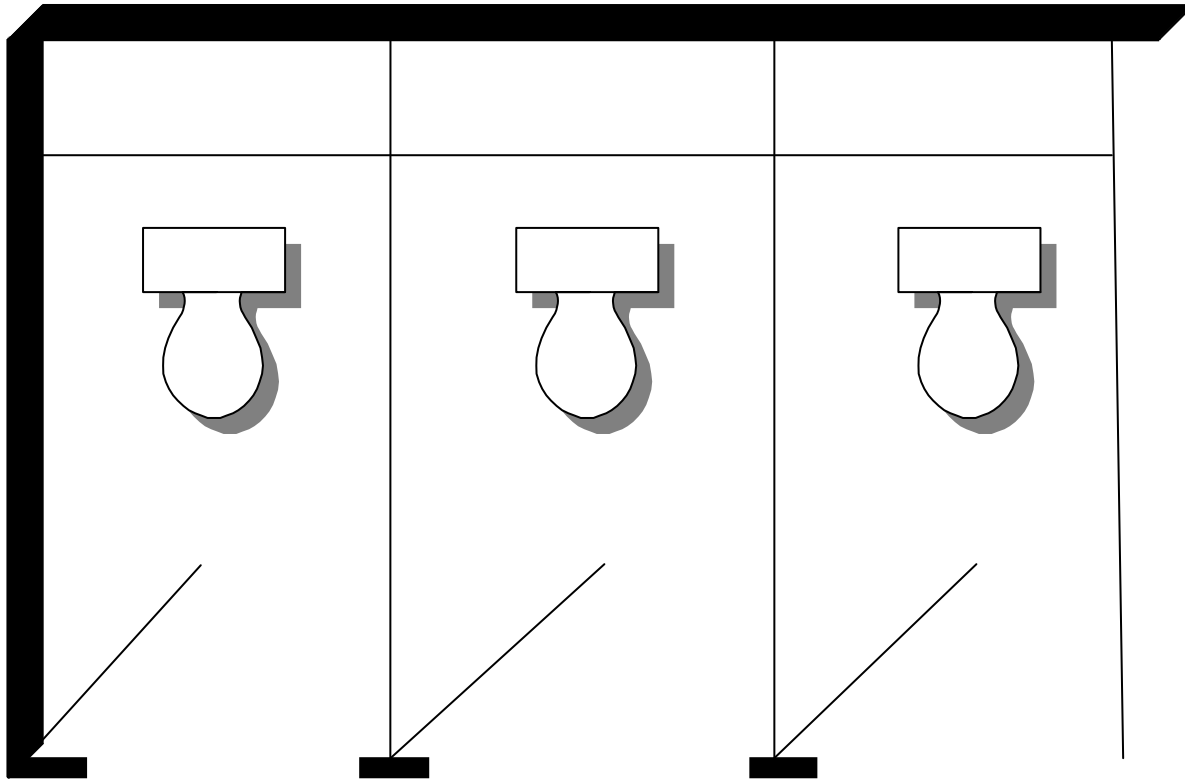
CUBICLES IN A CORNER LAYOUT SHOWING IPS AT THE BACK
